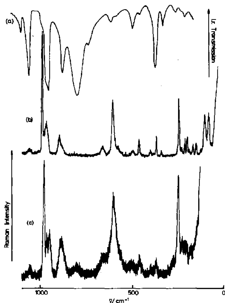
Fig. 7. Vibrational spectra of dodecamolybdates. (a) Infrared spectrum of \alpha -[(n-C 4 H 9 ) 4 N] 3 [PMo 12 O 40 ] KBr disc. (b) Raman spectrum of [(n-C 4 H 9 ) 4 N] 3 [PMo 12 O 40 ] KBr disc at ca. 80 K. (c) Raman spectrum of [(n-C 4 H 9 ) 4 N] 4 [PV V Mo 11 O 40 ] KBr disc at ca. 80 K. (a) Ref. 21, (b) and (c) Ref. 34.
