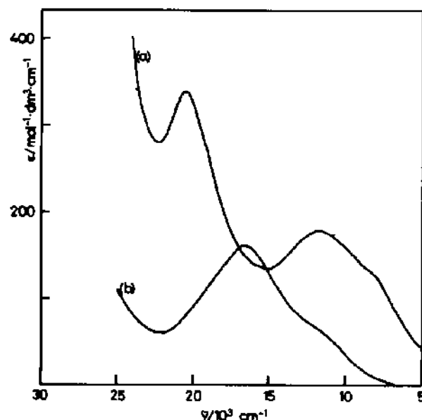
Fig. 9. Electronic spectra of one-electron reduced hexamolybdates. (a) [\text{Mo}_6\text{O}_{19}]^{3-} in DMF solution and (b) [\text{W}_5\text{MoO}_{19}]^{3-} in DMF solution. Ref. 70.
